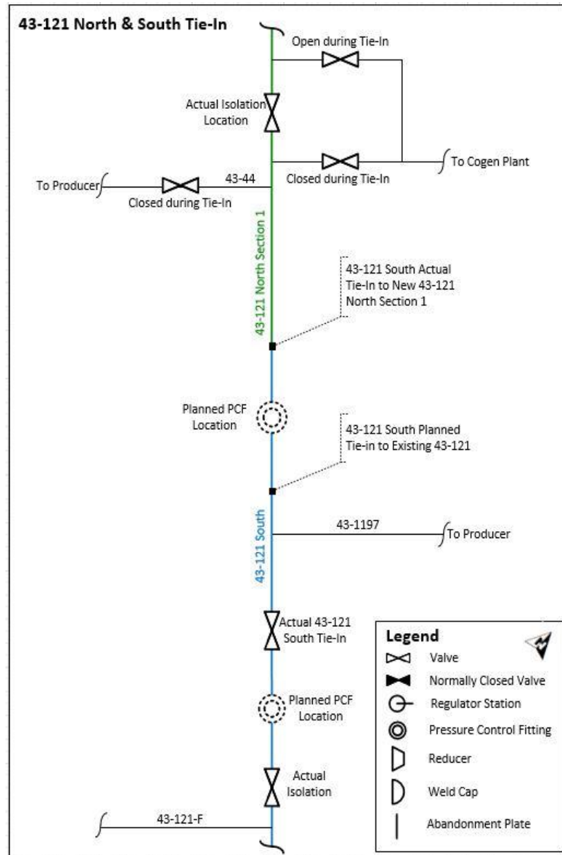
Figure 3: Supply Line 43-121 North and South Isolation Schematic
