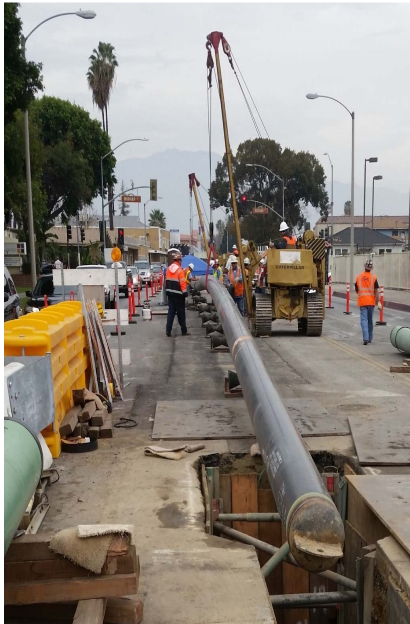
Figure 3: Shallow HDD Pullback Preparation at Santa Anita Avenue and MTA Way
