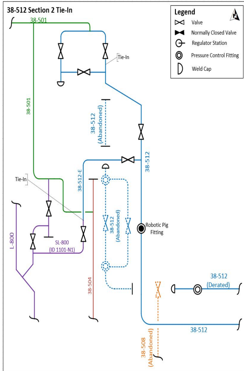
Figure 3: Schematic of the Supply Line 38-512 Section 2 Replacement Project
