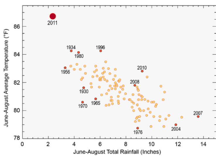
Figure 10.3. Graph shows average summer temperature and total rainfall in Texas from 1895 through 2012. The red dots illustrate the range of temperatures and rainfall observed over time. The record temperatures and drought during the summer of 2011 (large red dot) represent conditions far outside those that have occurred since the instrumental record began. 4 An analysis has shown that the probability of such an event has more than doubled as a result of human-induced climate change 3 . (Figure source: NOAA NCDC / CICS-NC).
