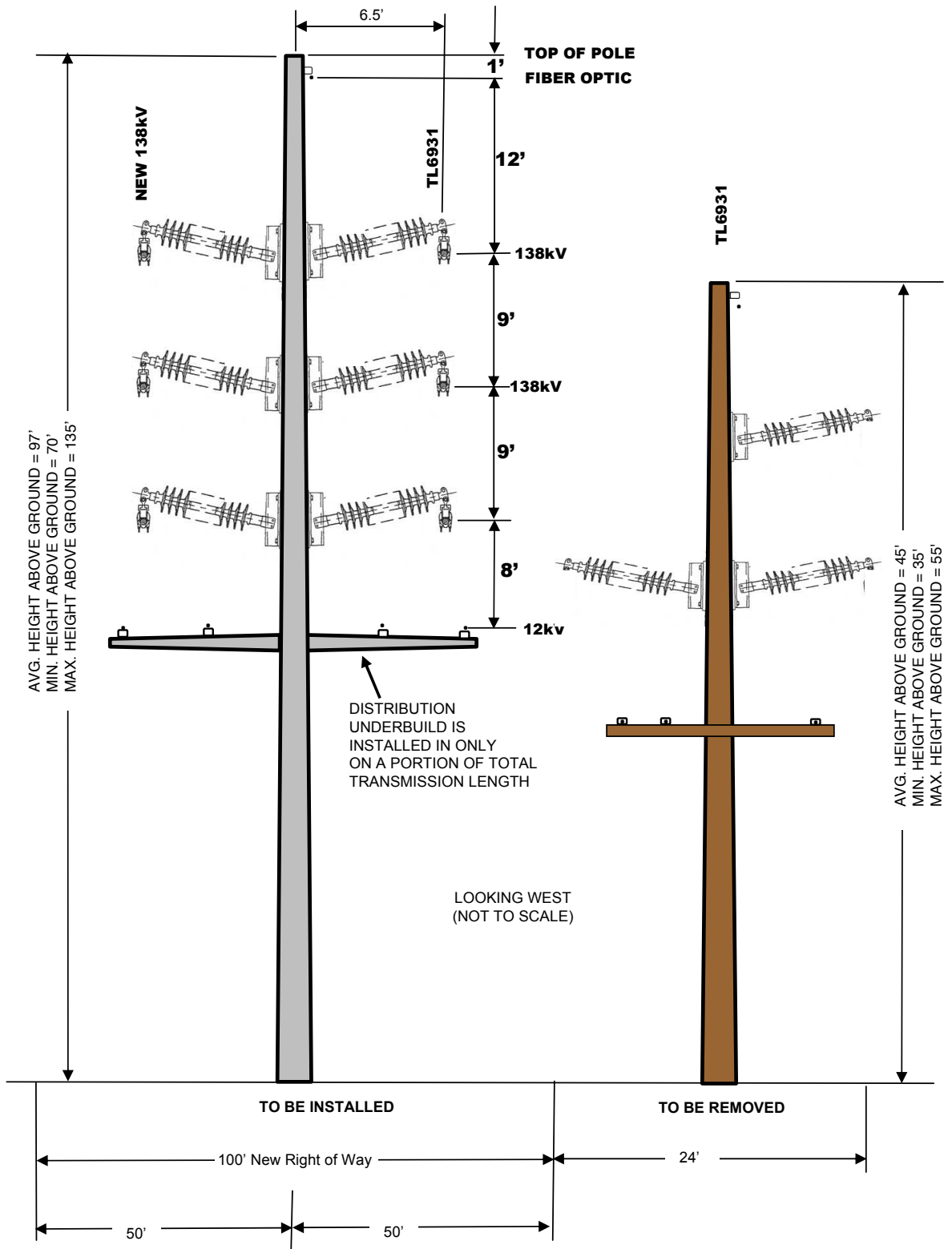
Figure 3-5 Cross Section A-A Typical 138 kV Double Circuit Tangent Steel Pole 12kV Underbuild
