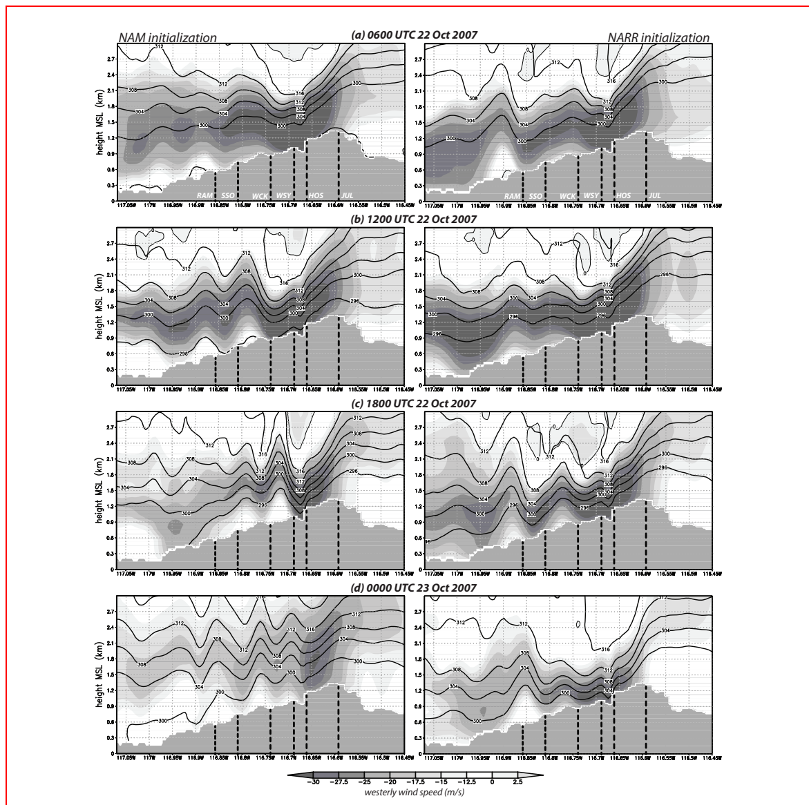
Fig. 20 Similar to Fig. 13, but for four times spanning the peak of the October 2007 event with runs initialized with NAM (left) and NARR (right).
