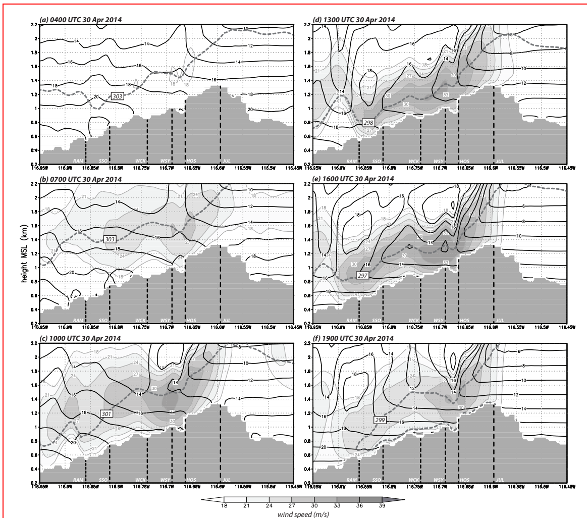
Fig. 14 West-east vertical cross-sections (longitude on abscissa) of full horizontal wind speed for six times during the late April 2014 event (shaded, with 3 \text{ m s}^{-1} interval grey contours), taken west-east across WSY with underlying topography in grey (see Fig. 6b). Black contours denote isotherms of temperature ( 2^\circ\text{C} interval). Grey dotted contours denote isentropes of virtual potential temperature. Approximate locations of stations JUL, HOS, WSY, WCK, SSO, and RAM are marked. WCK, SSO, JUL, RAM, and HOS are displaced somewhat from the vertical plane depicted.
