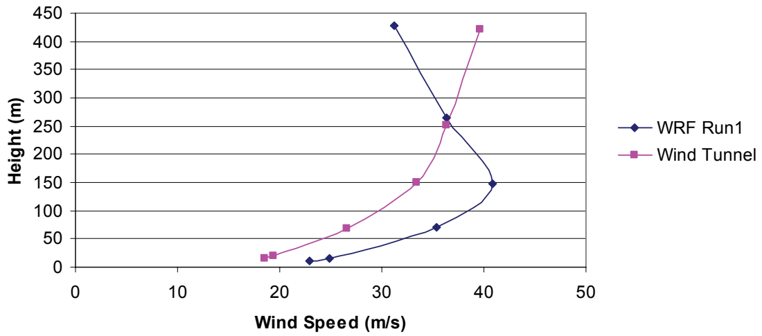
Exhibit 6. WRF wind speed profiles at the time of the peak 250m wind speed.
