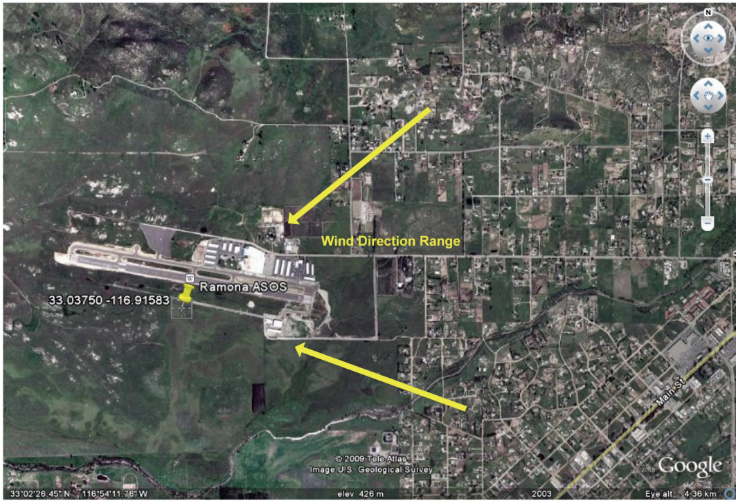
Exhibit 12a. Ramona Airport ASOS station location. Note suburban development upwind for the Santa Ana event and airport buildings upwind causing some shielding.
