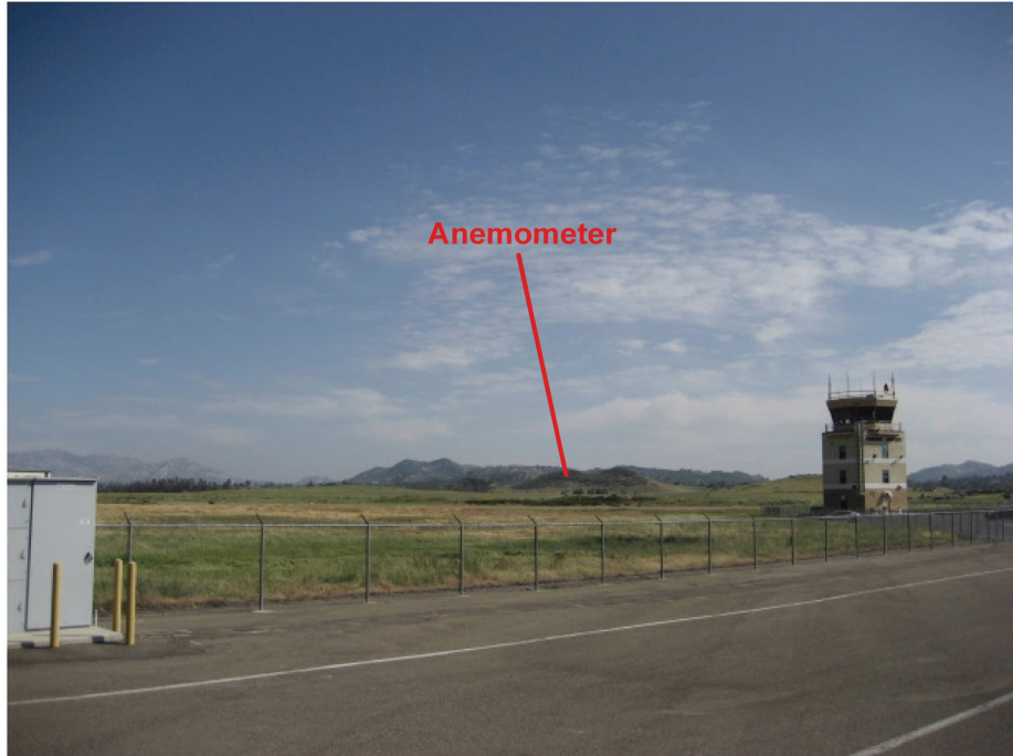
Exhibit 12c. Photo of Ramona ASOS from location KRNM1 (see Exhibit 12b).
