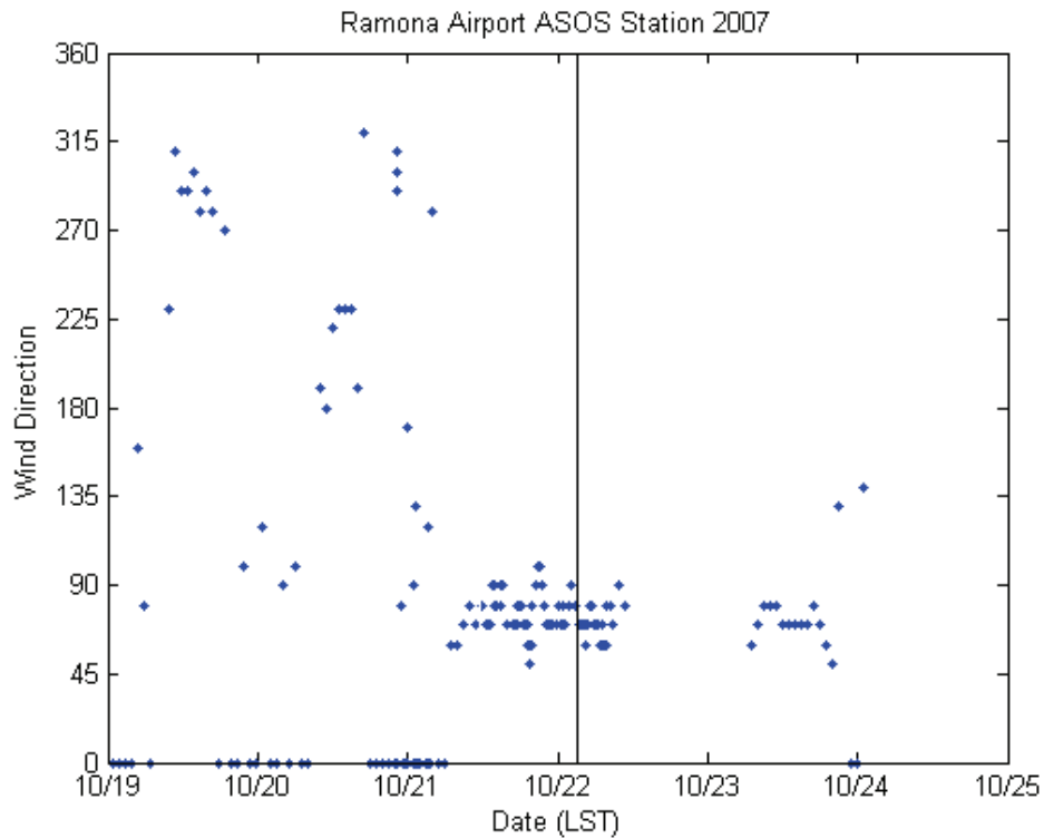
Exhibit 12f. Wind direction time histories for Ramona Airport during the Santa Ana event. The black line indicates the Rice Canyon fire initiation time.
