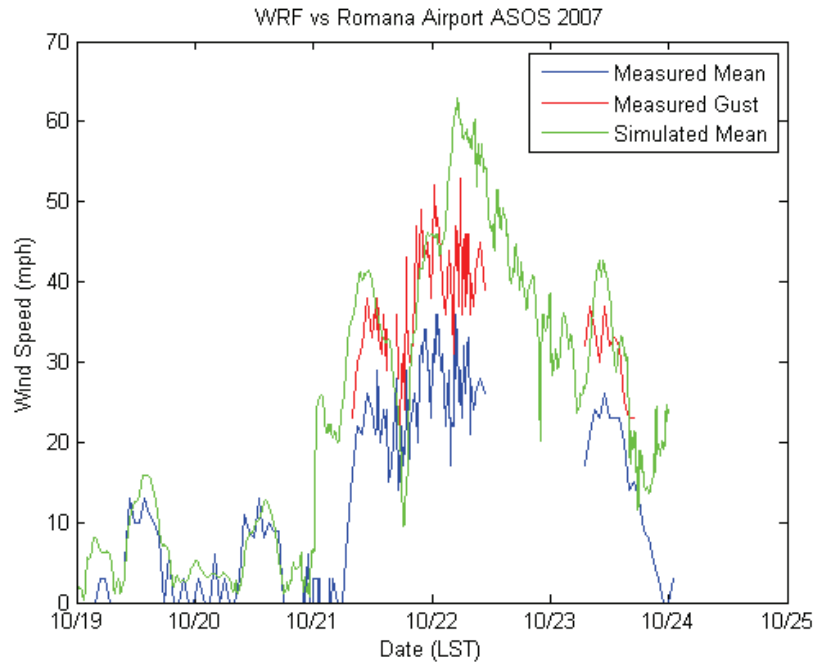
Exhibit 12h. Mean and gust speed time histories for Ramona Airport with WRF mean wind speeds imposed.
