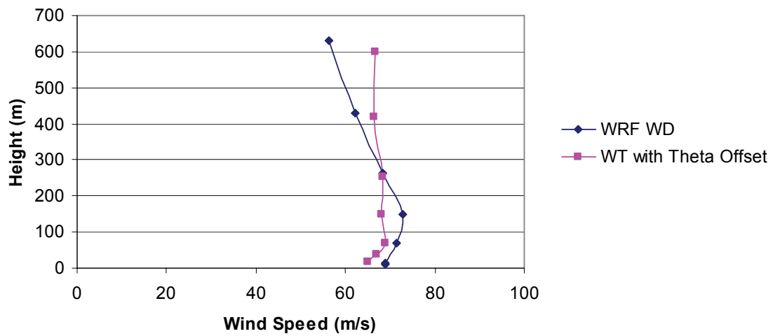
Exhibit 8. WRF wind direction profiles at the time of the peak 250m wind speed.
