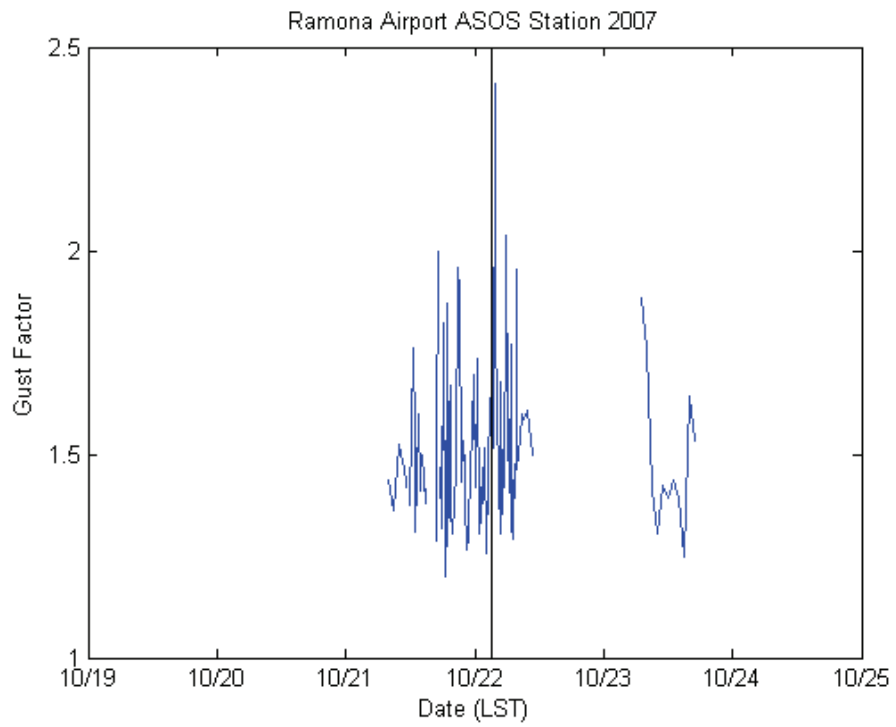
Exhibit 12g. Gust factor time history for Ramona Airport during the Santa Ana event. The black line indicates the Rice Canyon fire initiation time.
