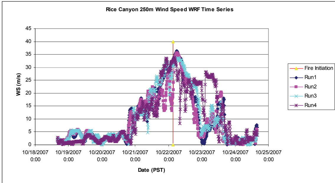
Exhibit 4. WRF 250m wind speed time histories for all four runs.
