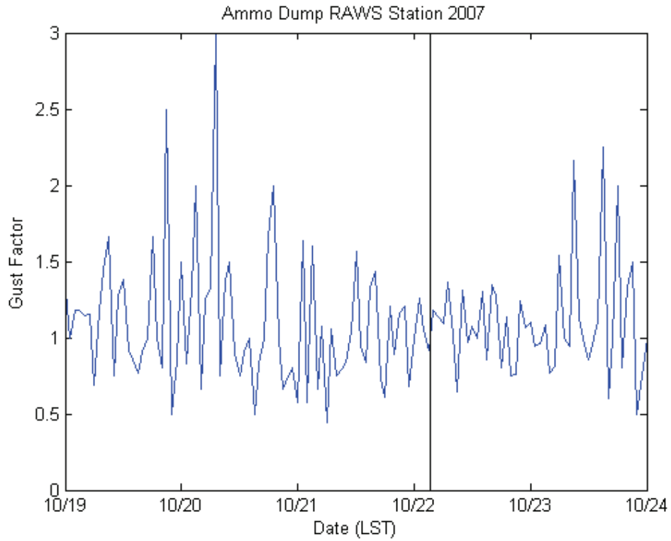
Exhibit 11c. Gust factor time history for Ammo Dump during the Santa Ana event. The black line indicates the Rice Canyon fire initiation time.
