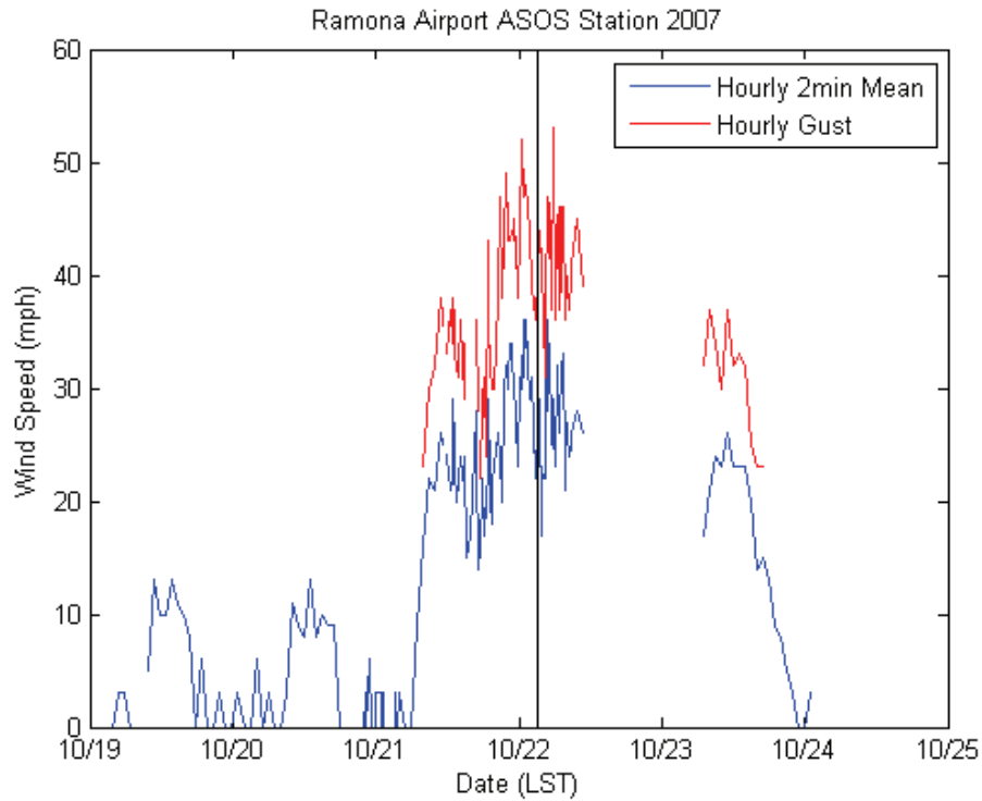
Exhibit 12e. Mean and gust speed time histories for Ramona Airport during the Santa Ana event. The black line indicates the Rice Canyon fire initiation time.
