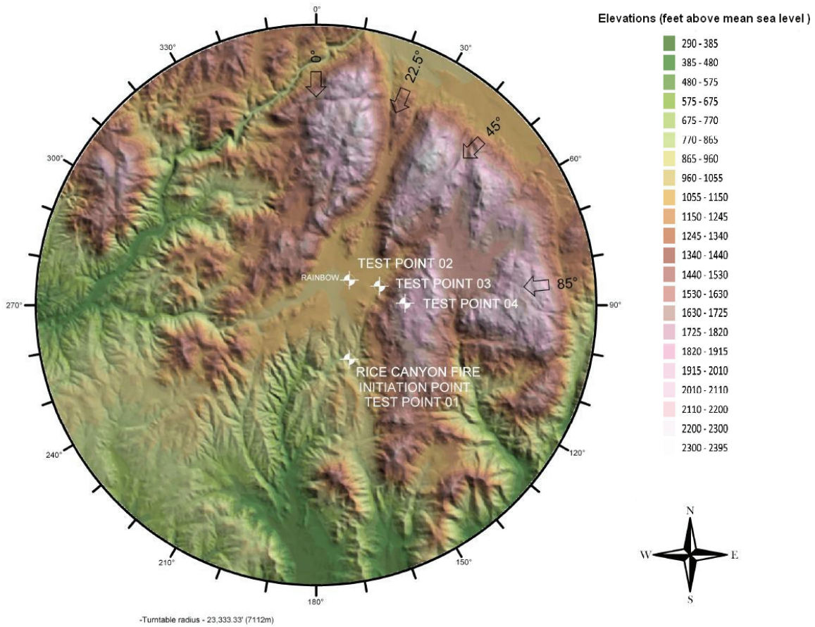
Exhibit 3b. Rice Canyon wind tunnel model test turntable with upwind terrain.
