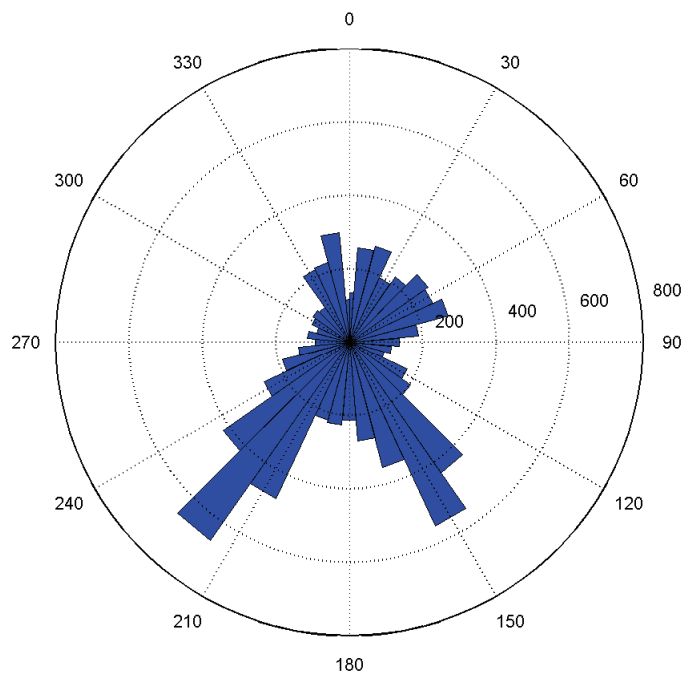
Exhibit 11d. Wind rose for Ammo Dump from 2007.
