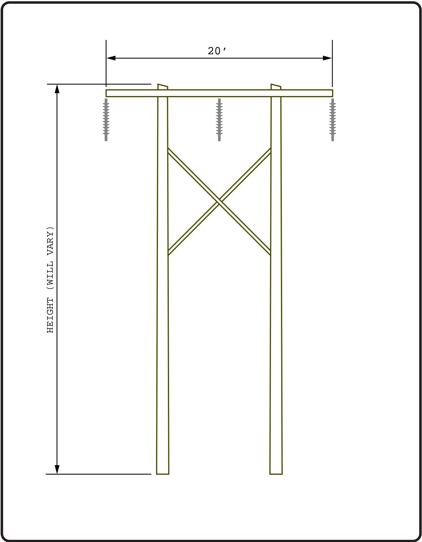
Existing Wood H-Frame Distribution Pole
