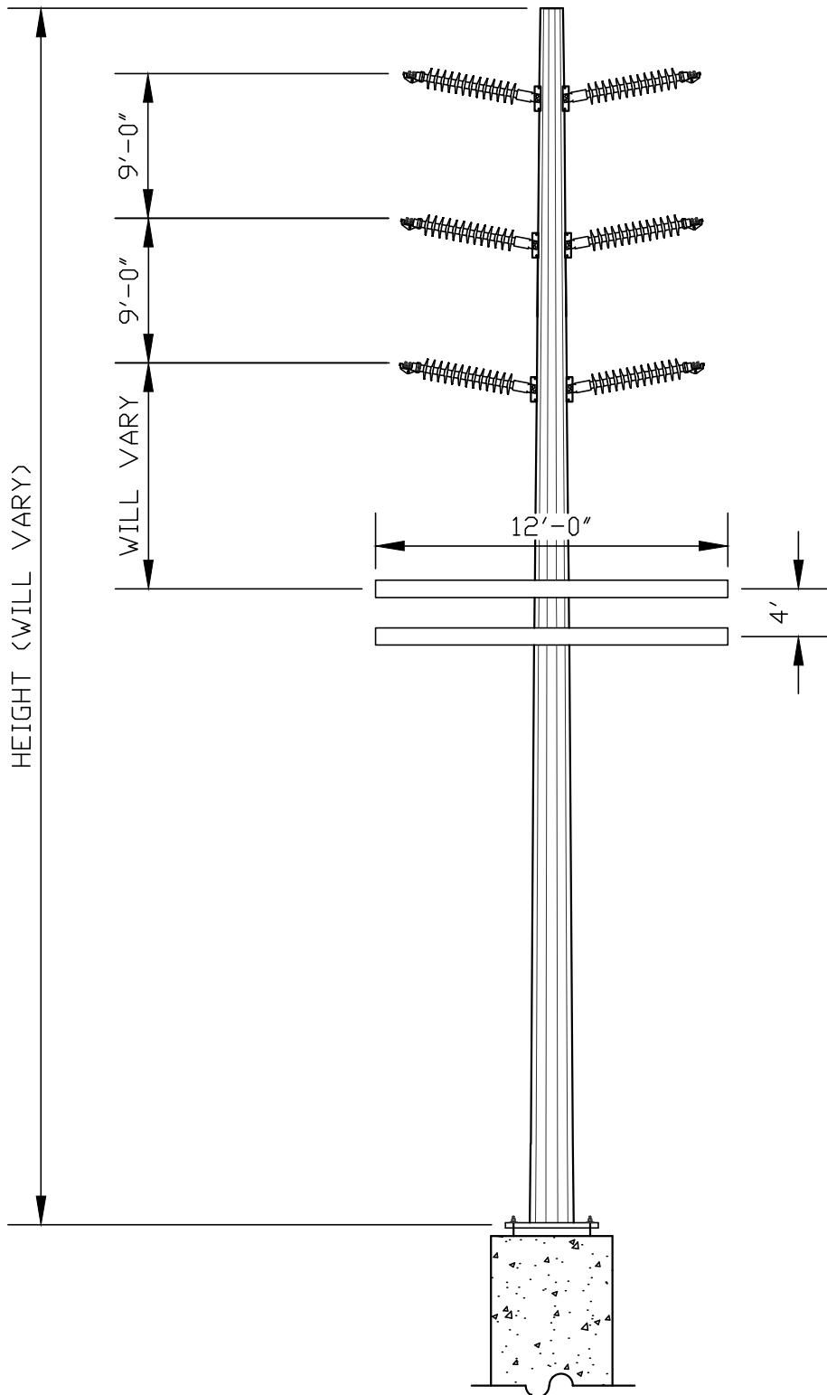
Proposed Double-Circuit Tangent Transmission Pole
