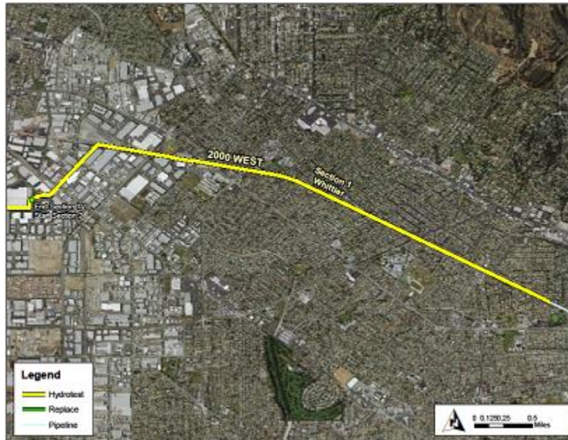
Figure 4: Satellite Image of L-2000 West Hydrotest Project - Section 1 Whittier
