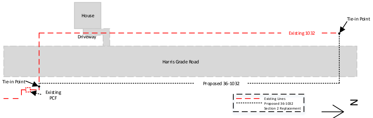
Figure 12: Stage 4 SL-36-1032 Section 2
