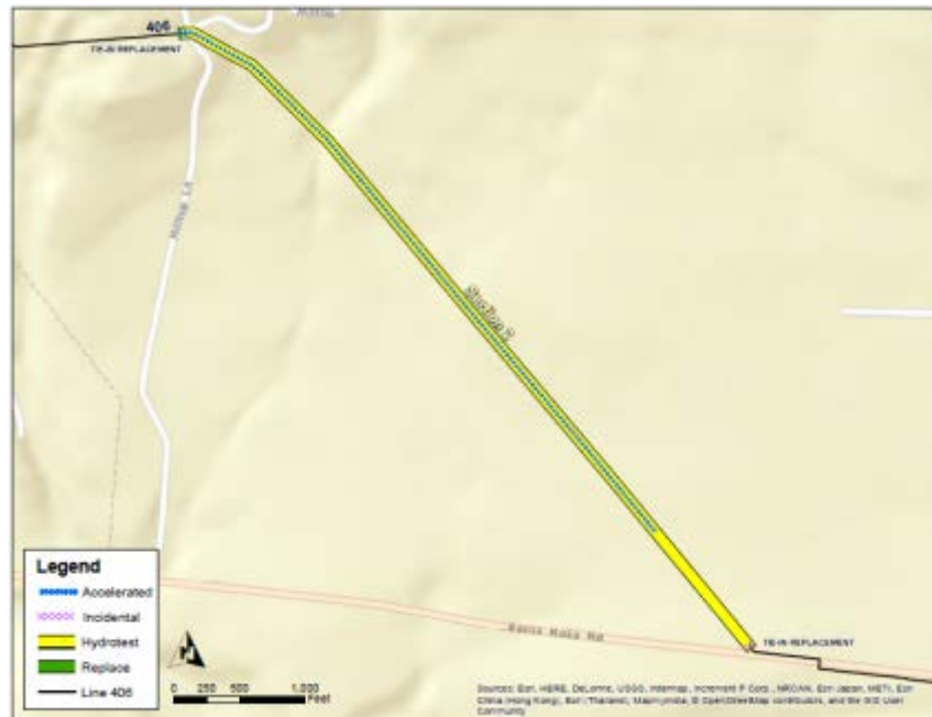
Figure 5: Overview Map of L-406 Section 2 Hydrotest Project
